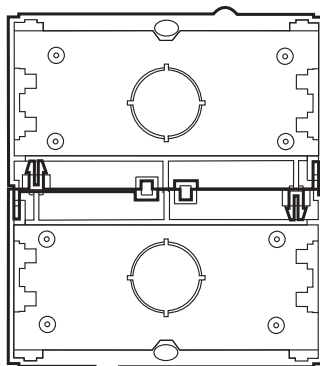
9740005 CMO-002 114 x 131 x 45 mm
